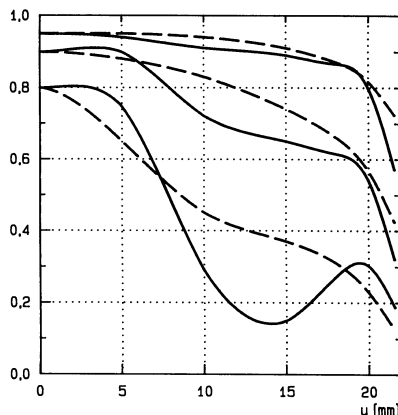
T f-number k = 5.6
