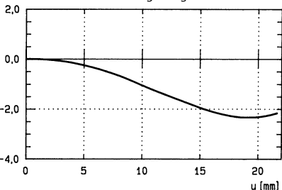
v Distortion in % of image height u
